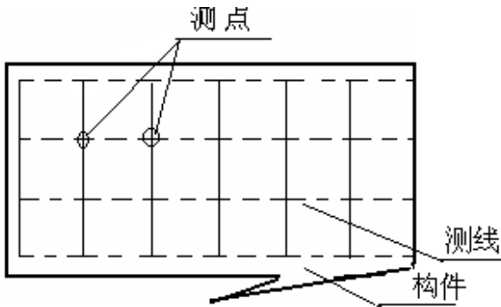
图 5-3 测区测点布置
